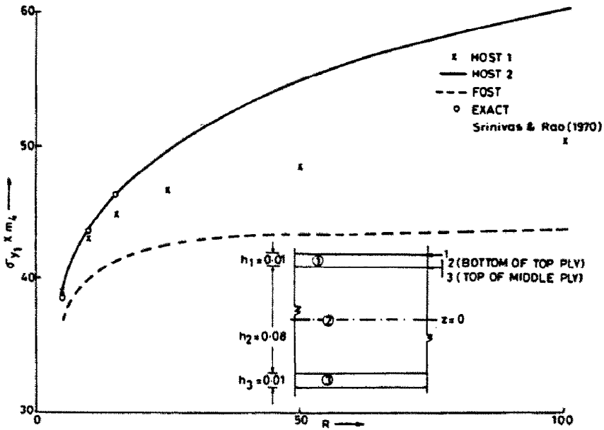
Fig. 5. Effect of modular ratio (top or bottom/middle) on maximum inplane normal stress (at level 1 in y-direction) for a simply supported, symmetrically laminated square plate under uniform transverse load ( a/h = 10 ).
