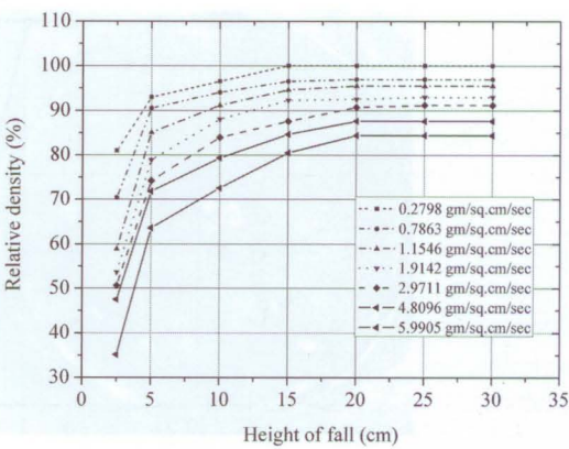
Fig. 5 Effect of deposition intensity and height of fall on relative density - Sand Grade III
