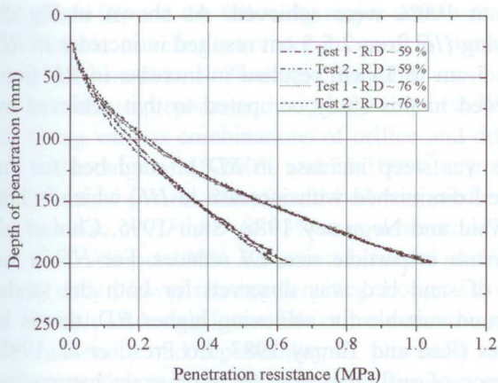
Fig. 7 Results of CPT for evaluation of repeatability and uniformity pluviated bed - Sand Grade II
