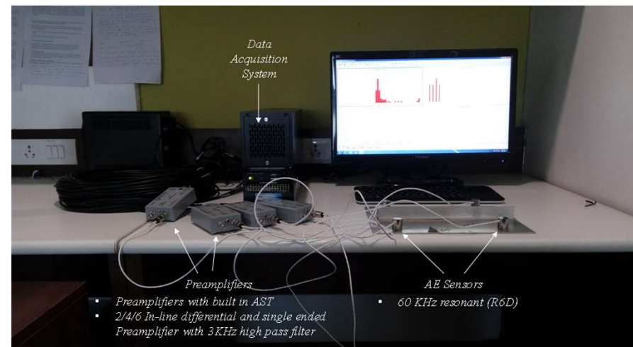
Physical Acoustics AE System (8 Channel)
