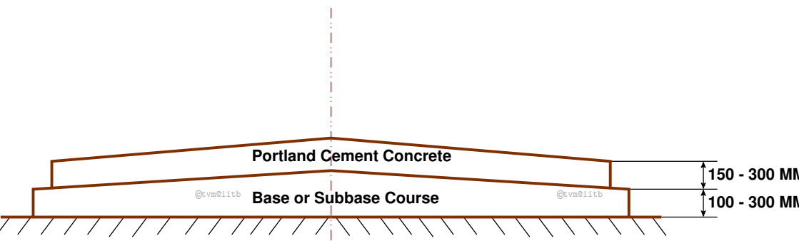
Figure 3: Typical Cross section of Rigid pavement
