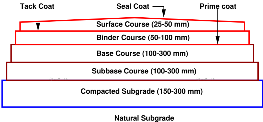
Figure 2: Typical cross section of a flexible pavement
