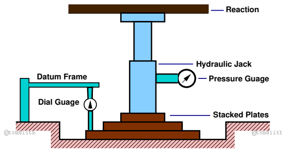
Figure 3: Plate load test
