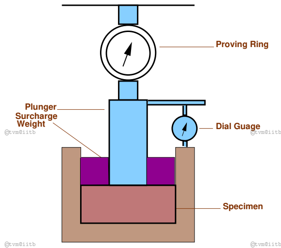
Figure 2: CBR Test
