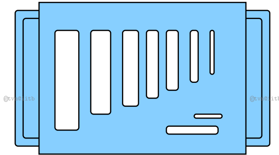
Figure 4: Flakiness gauge
