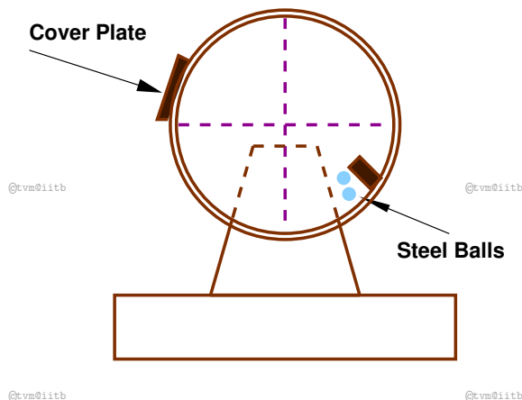
Figure 2: Los Angeles abrasion test setup
