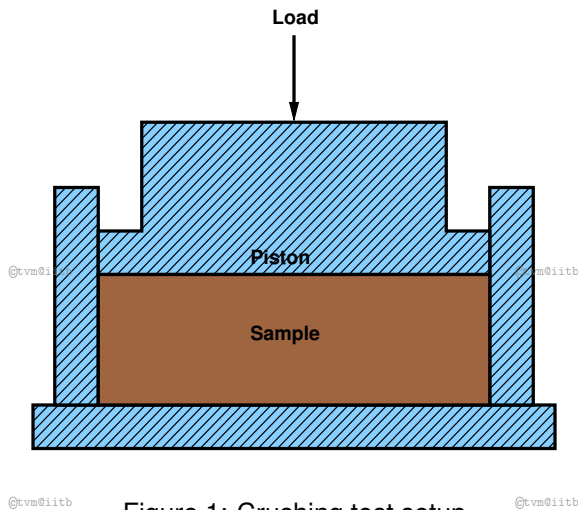
Figure 1: Crushing test setup
