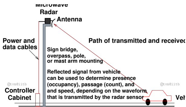
Figure 5: Microwave radar operation. Source
