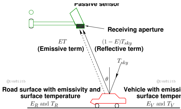
Figure 3: Emission and reflection of energy by vehicle and road surface. (Source: FHWA vehicle detection manual)
