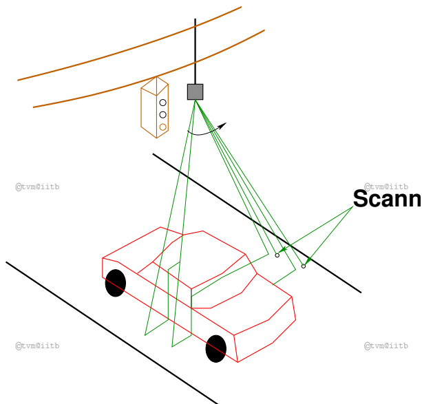
Figure 4: Laser radar beam geometry. (Source: FHWA vehicle detection manual)
