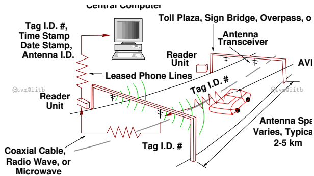
Figure 2: AVI Vehicle-to-Roadside Communication Process, Source: Travel Time Detection Hand Book, [16]
