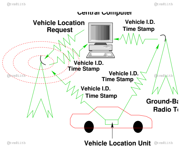
Figure 3: Ground-Based Radio Navigation Communication Process, Source: Travel Time Detection Hand Book, [16]
