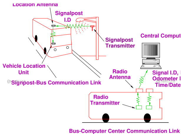
Figure 1: Signpost-Based AVL Communication Processes, Source: Travel Time Detection Hand Book, [16]
