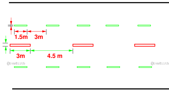
Figure 2: Center line and lane marking for a four lane road
