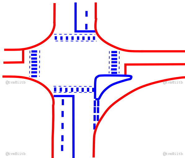
Figure 11: Pedestrian marking near an intersection
