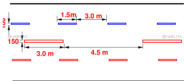
Figure 6: Traffic lane marking for a four lane road with broken center line
