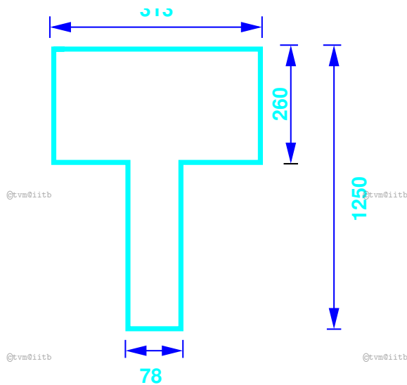
Figure 14: Typical dimension of the character T used in road marking
