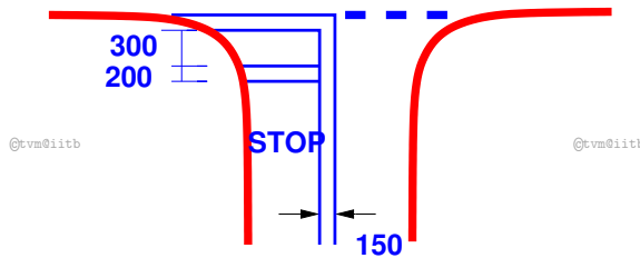
Figure 10: Stop line marking near an intersection
