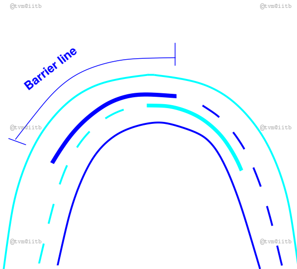
Figure 8: No passing zone marking at horizontal curves
