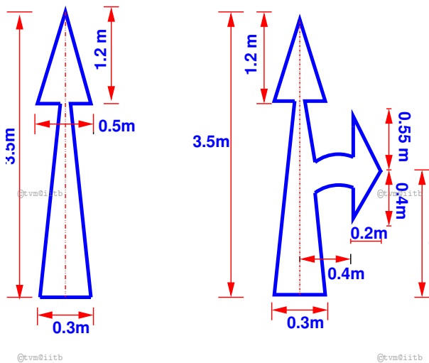
Figure 12: Directional arrow marking
