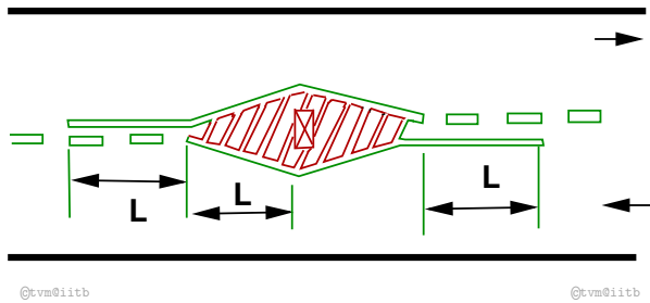
Figure 15: Approach marking for obstructions on the road way
