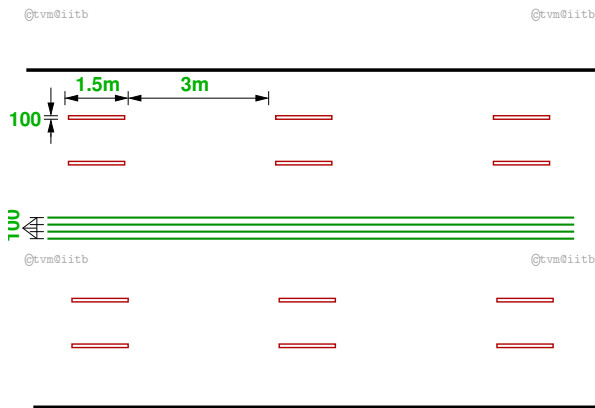
Figure 3: Double solid line for a two lane road
