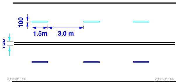
Figure 5: Lane marking for a four lane road with solid barrier line
