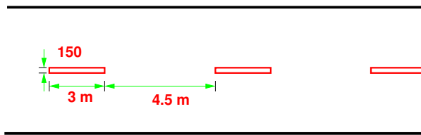
Figure 1: Center line marking for a two lane road
