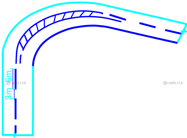
Figure 9: Warning line marking for a two lane road
