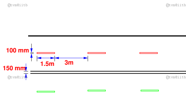
Figure 3: Double solid line for a two lane road
