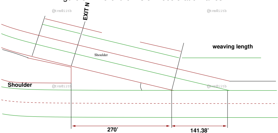
Figure 3: Different forms of Deceleration lanes
