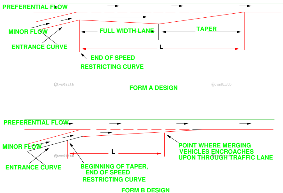
Figure 1: Different forms of Acceleration lanes
