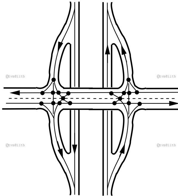
@tvm@iitb Figure 6: Diamond interchange @tvm@iitb
