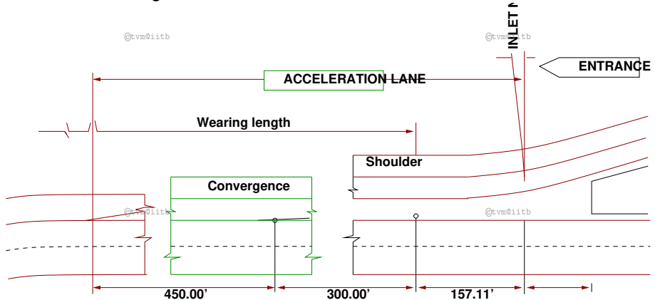
Figure 1: Different forms of Acceleration lanes
