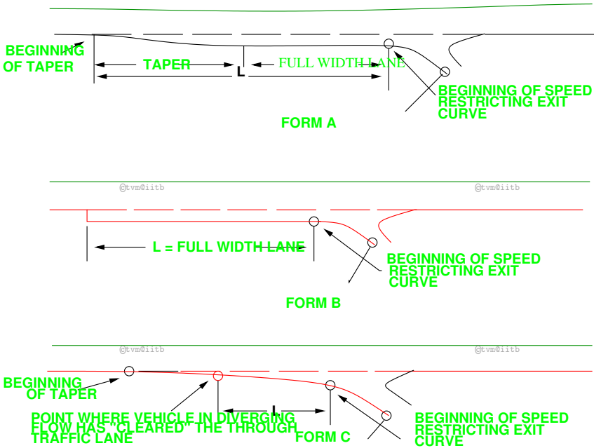
Figure 3: Different forms of Deceleration lanes
