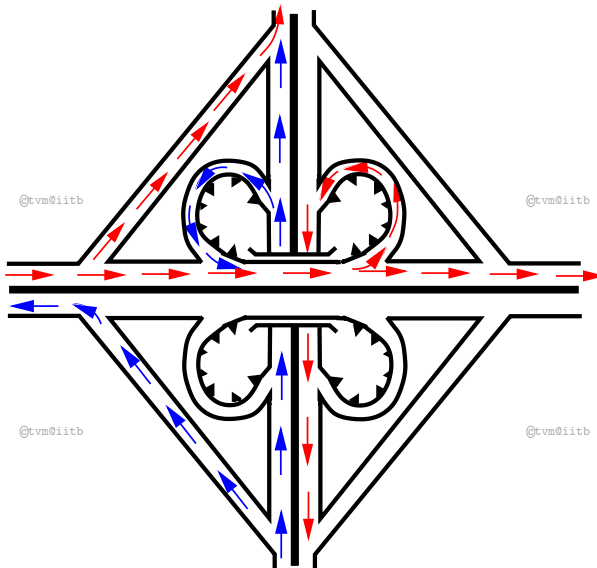
Figure 7: Cloverleaf interchange
