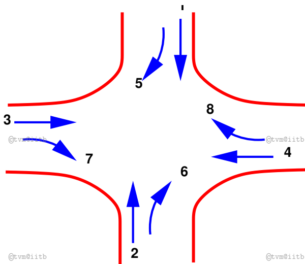
Figure 1: Four legged intersection
