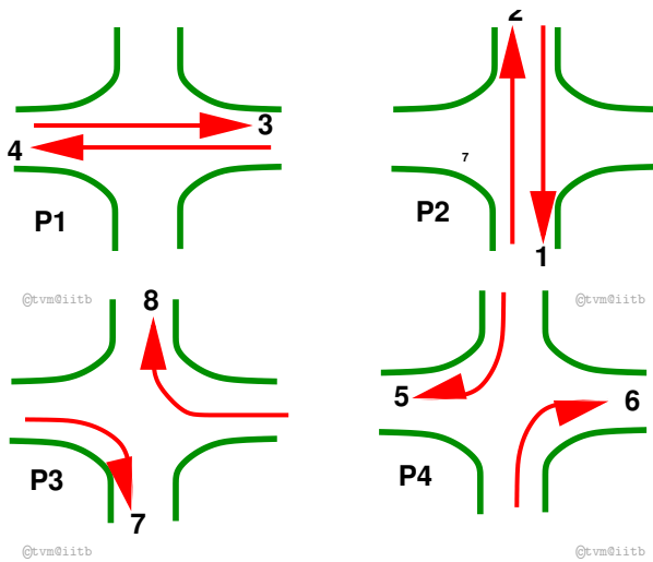
Figure 4: Movements in four phase signal system: option 2
