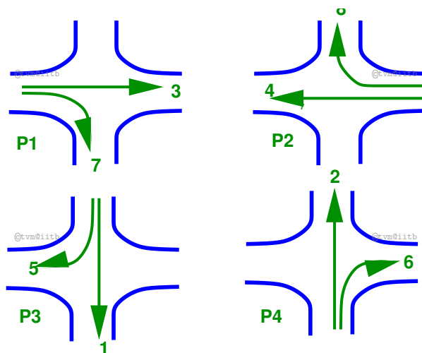
Figure 3: Movements in four phase signal system: option 1
