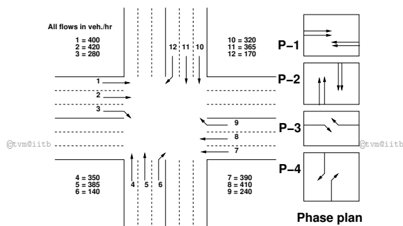
Figure 14: Intersection flows and phase plan
