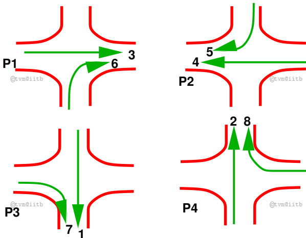
Figure 5: Movements in four phase signal system: option 3
