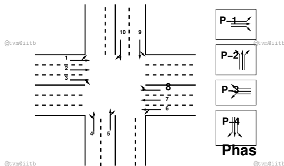
Figure 15: Intersection flows and phase plan
