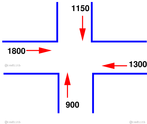
Figure 8: Numerical example-2: Traffic flow in the intersection
