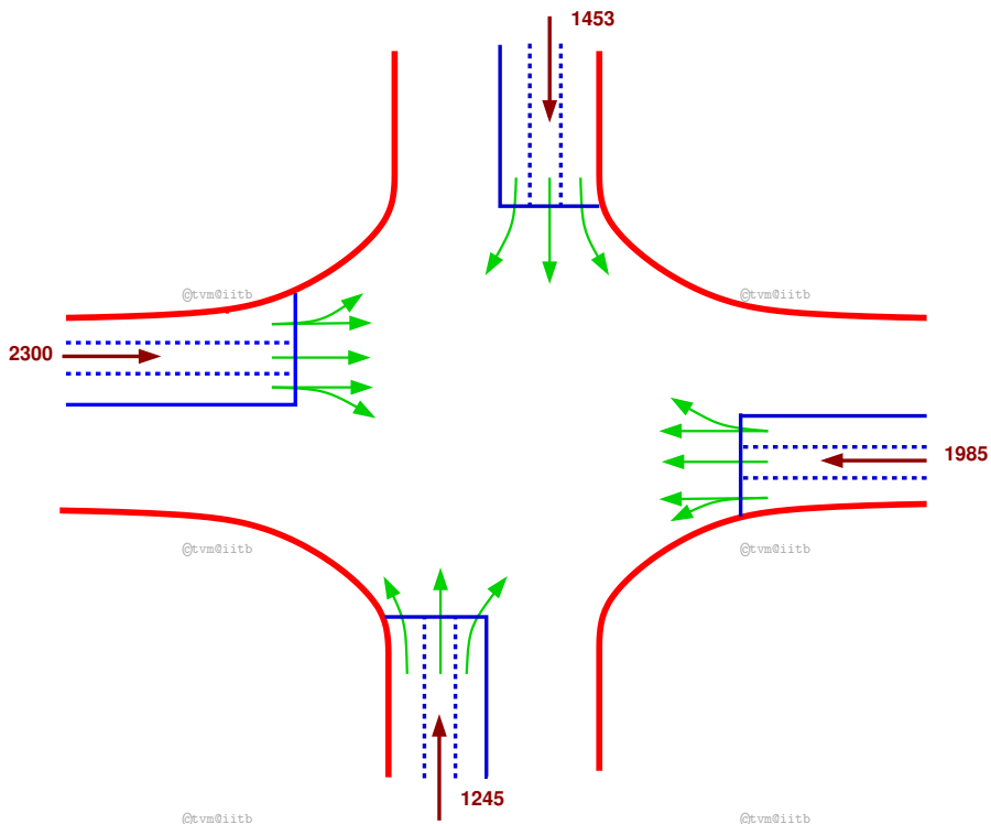
Figure 1: Numerical example: Flow details
