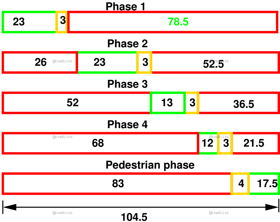
Figure 5: Timing diagram
