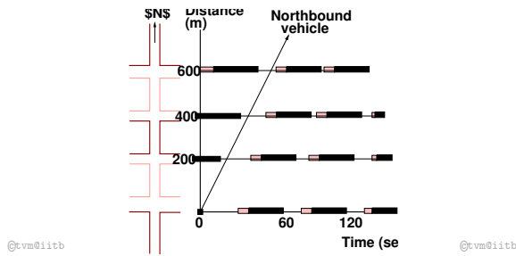
Figure 2: Time space diagram
