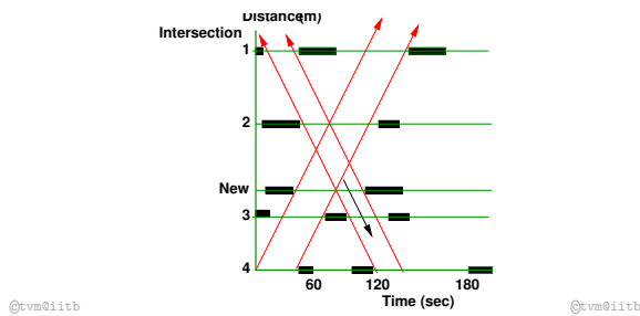
Figure 12: Effect of inserting a new signal into system
