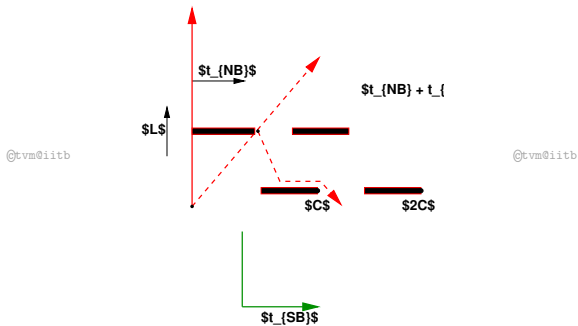
Figure 7: Offsets on 2 way arterial are not independent- One cycle length
