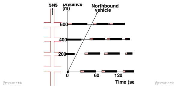
Figure 3: Case study:progression on a one way street
