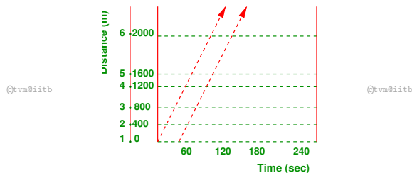
Figure 5: Vehicle trajectory and green wave in a progressed movement
