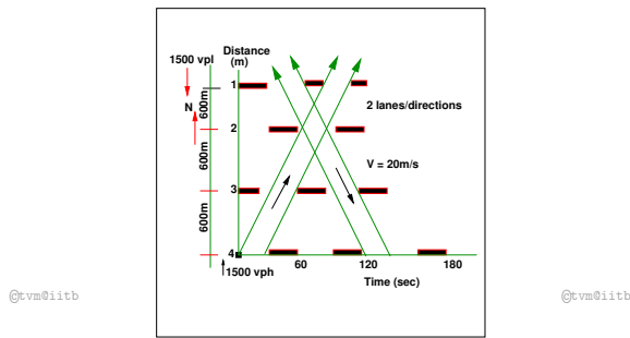
Figure 11: Case study: Four intersections with good progressions
