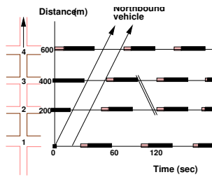
Figure 10: Bandwidths on a time space diagram
