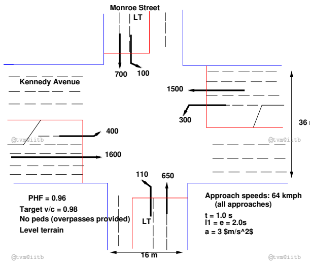
Figure 5: Intersection for the Example
