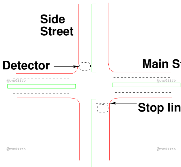
Figure 3: Semi-Actuated Control
