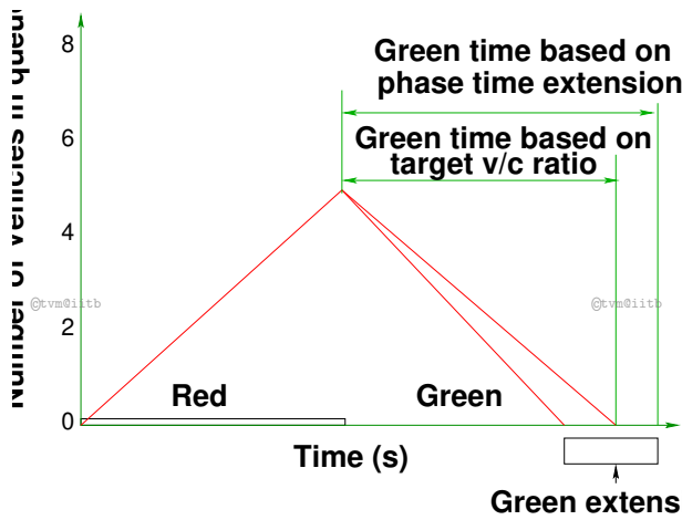
Figure 1: Queue accumulation polygon illustrating two methods of green time computation
