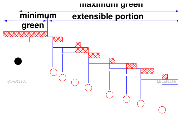
Figure 2: Operation of an Actuated Phase
