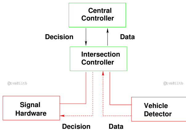
Figure 3: Communication Network (Source: Muralidharan, 2006)
