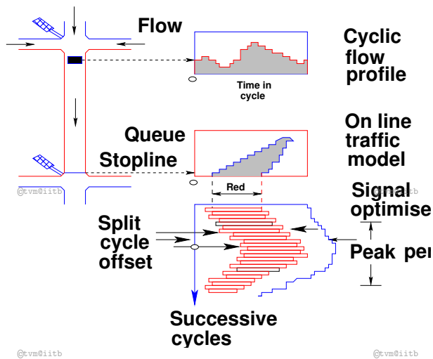
Figure 5: Key elements of the SCOOT ATC system (Source: Dennis I. Robertson and R. David Bretherton 1991)
