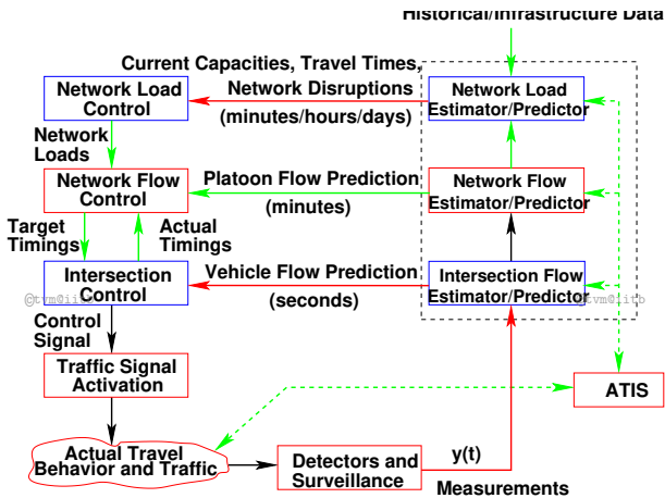
Figure 4: Area traffic control architecture (Source: Pitu B. Mirchandani, K. Larry Head, 1998)
