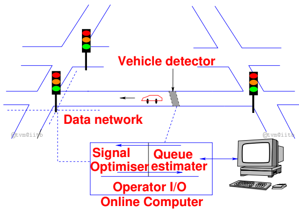
Figure 6: Working Principle of SCOOT (Source: www.scoot-utc.com )
