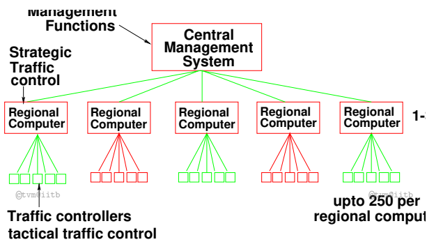
Figure 7: Shows the SCAT Computer Hierarchy (Source: Lowrie, 1982)
