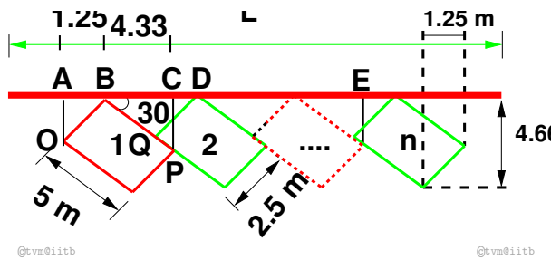
Figure 2: Illustration of 30° parking
