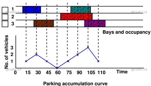
Figure 7: Parking bays and accumulation curve
