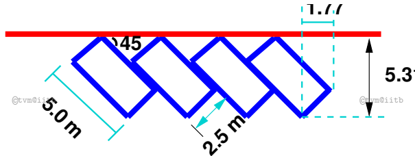
Figure 3: Illustration of 45° parking
