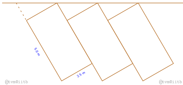
Figure 4: Illustration of 60° parking
