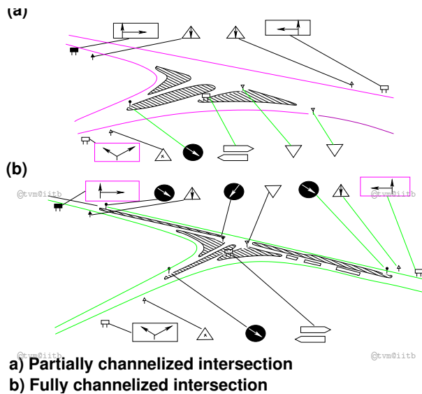
Figure 15: Channelized Intersection ensuring safety
