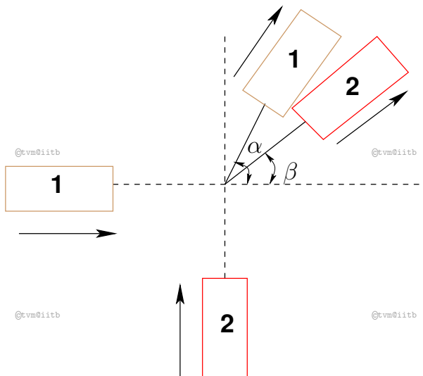
Figure 9: After collision movement of car 1 and car 2 in north of east
