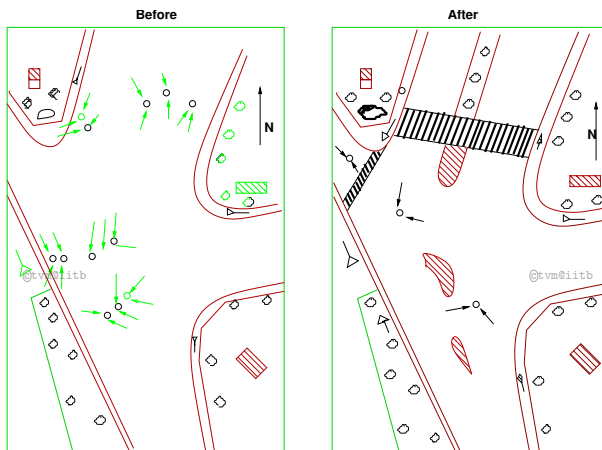
Figure 13: Diagram of accidents before and after reconstruction
