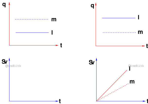
Figure 2: Constant arrival and service rates
