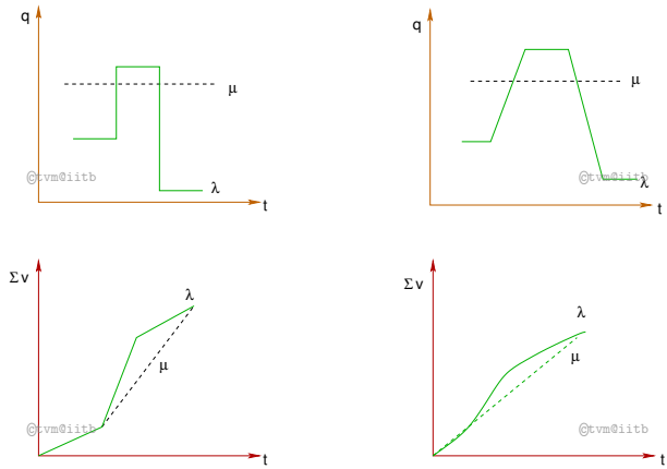
Figure 4: Varying arrival rate and constant service rate
