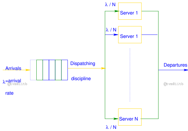
Figure 6: Multi-server model
