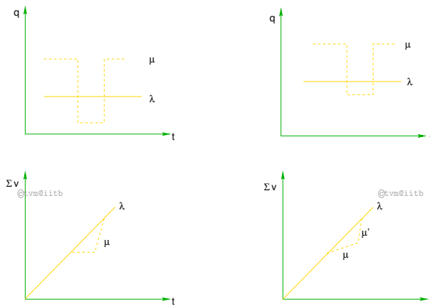
Figure 3: Constant arrival rate and varying service rate
