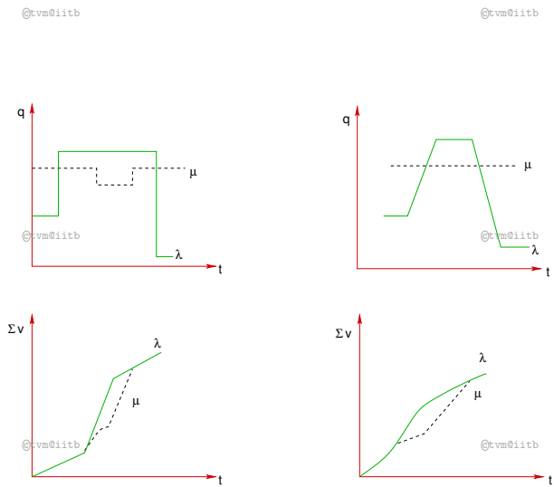
Figure 5: Varying arrival and service rates
