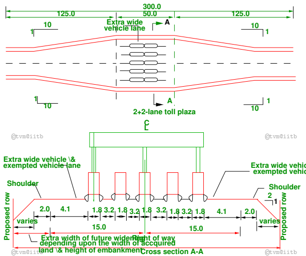
Figure 5: General Layout 2+2 lane Toll Plaza (Source: [3])
