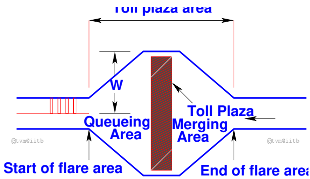
Figure 3: Toll Plaza Geometry
