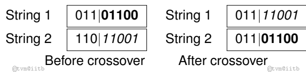
Figure 5: One site crossover operation
