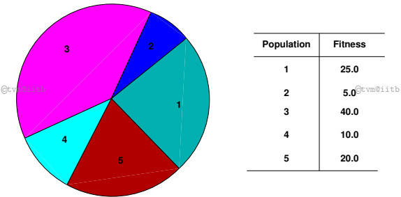
Figure 4: A roulette-wheel marked for five individuals according to their fitness values. Third individual has a higher probability of selection than any other
