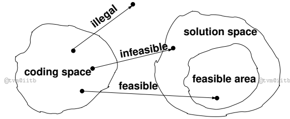
Figure 3: Coding in GA
