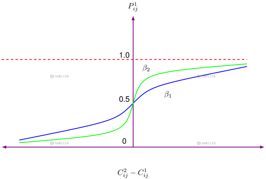
Figure 1: Logit Function
