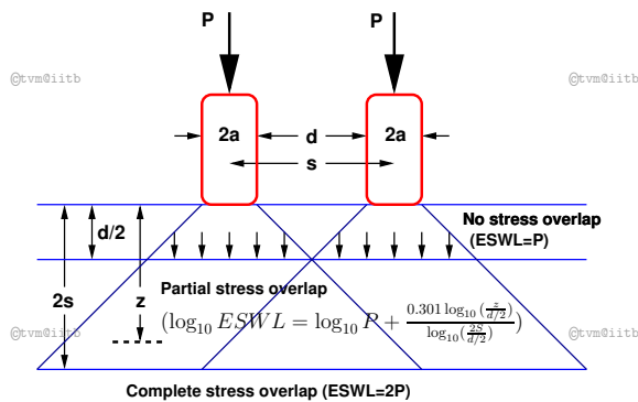
Figure 1: ESWL-Equal stress concept
