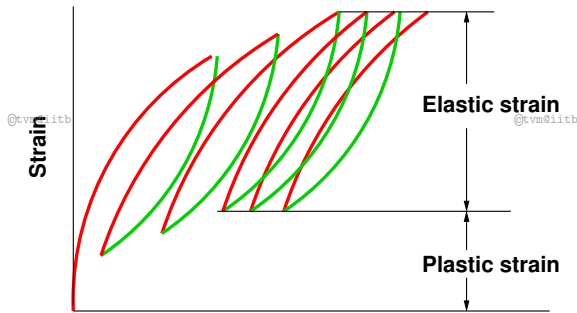
Figure 2: Recoverable strain under repeated loads
