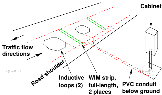
Figure 4: WIM installation with full-length piezoelectric sensors Source: FHWA vehicle detection manual
