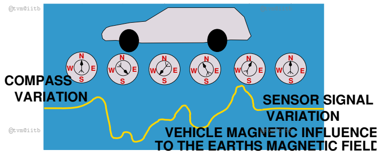
(b) Perturbation of Earth's magnetic field by a ferrous vehicle
