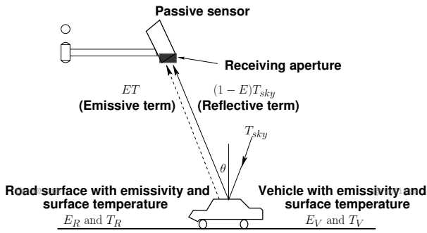
Figure 6: Emission and reflection of energy by vehicle and road surface. (Source: FHWA vehicle detection manual)
