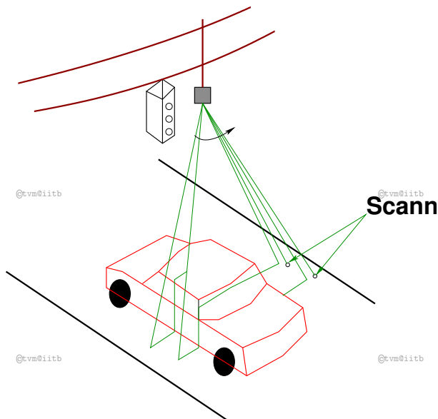
Figure 7: Laser radar beam geometry. (Source: FHWA vehicle detection manual)
