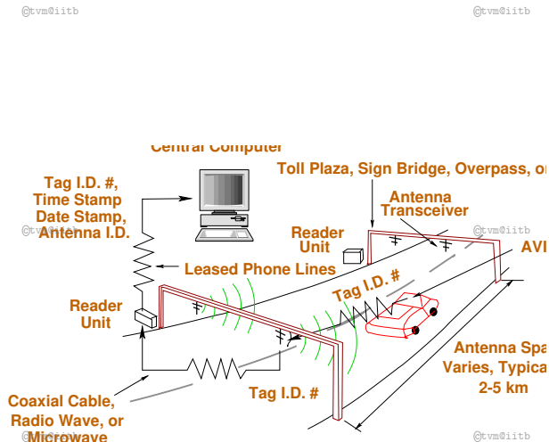
Figure 13: AVI Vehicle-to-Roadside Communication Process, Source: Travel Time Detection Hand Book
