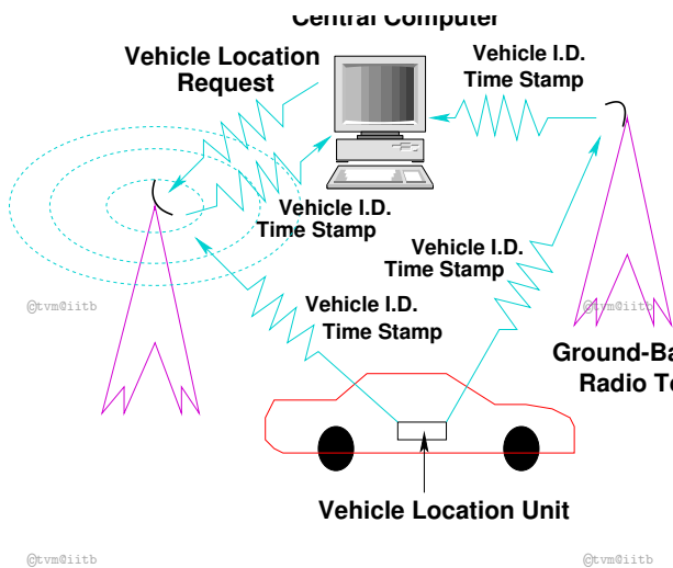
Figure 14: Ground-Based Radio Navigation Communication Process, Source: Travel Time Detection Hand Book
