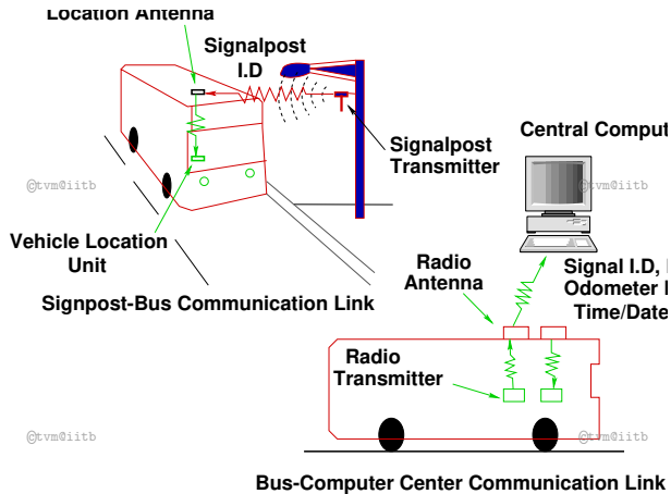
Figure 12: Signpost-Based AVL Communication Processes, Source: Travel Time Detection Hand Book
