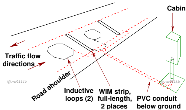
Figure 8: WIM installation with full-length piezoelectric sensors Source: FHWA vehicle detection manual
