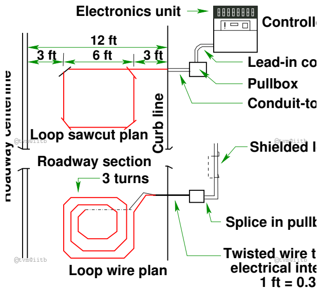
Figure 3: Schematic diagram of single loop detectors, source
