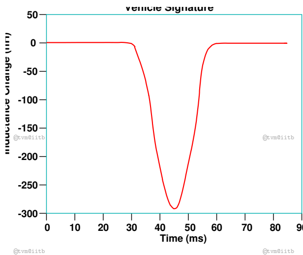
Figure 6: Inductive waveform of a typical passenger car, source
