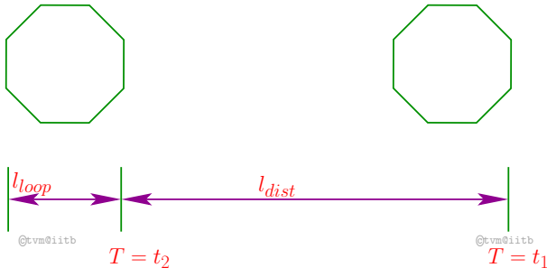
Figure 4: Schematic diagram of dual loop detectors
