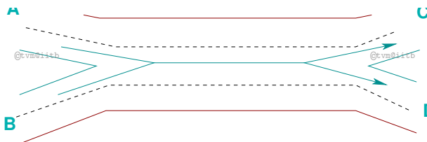
Figure 13: Major Weave with Merge at Entry Gore and Lane Balance at Exit Gore
