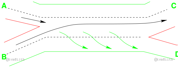
Figure 12: Major Weave with Merge at Entry Gore
