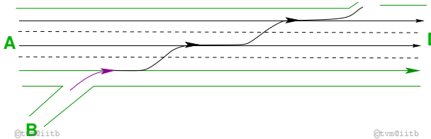
Figure 15: Two-Sided Weave
